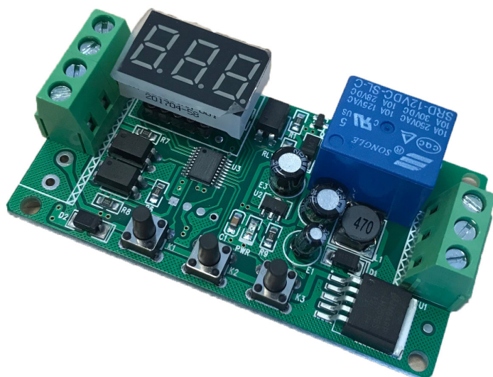
Timer Relay
