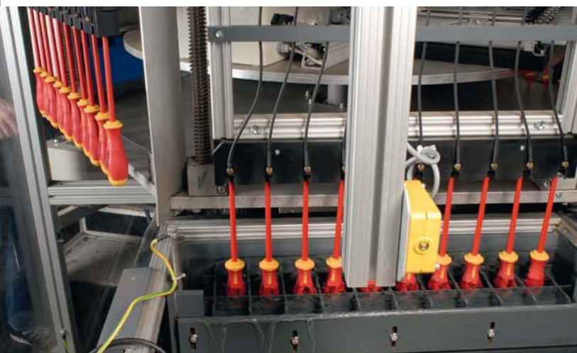
100% testing (10.000 V)
