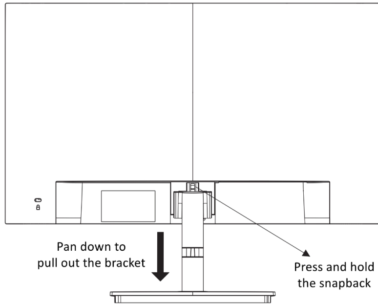
Figure 2-4 Remove the Device and Bracket
