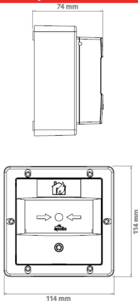
Figure 2: Waterproof Addressable Manual Call Point dimensional drawing
