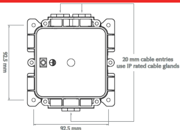
Figure 1: Waterproof Addressable Manual Call Point Backbox
