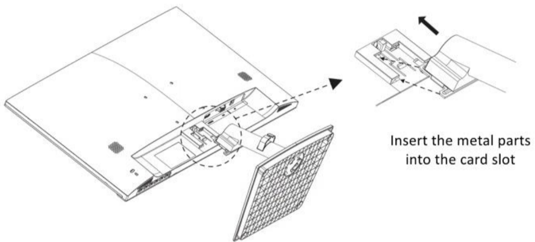
Figure 2-4 Insert the Metal Parts (Model A)
