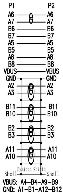
Circuit Configuration
