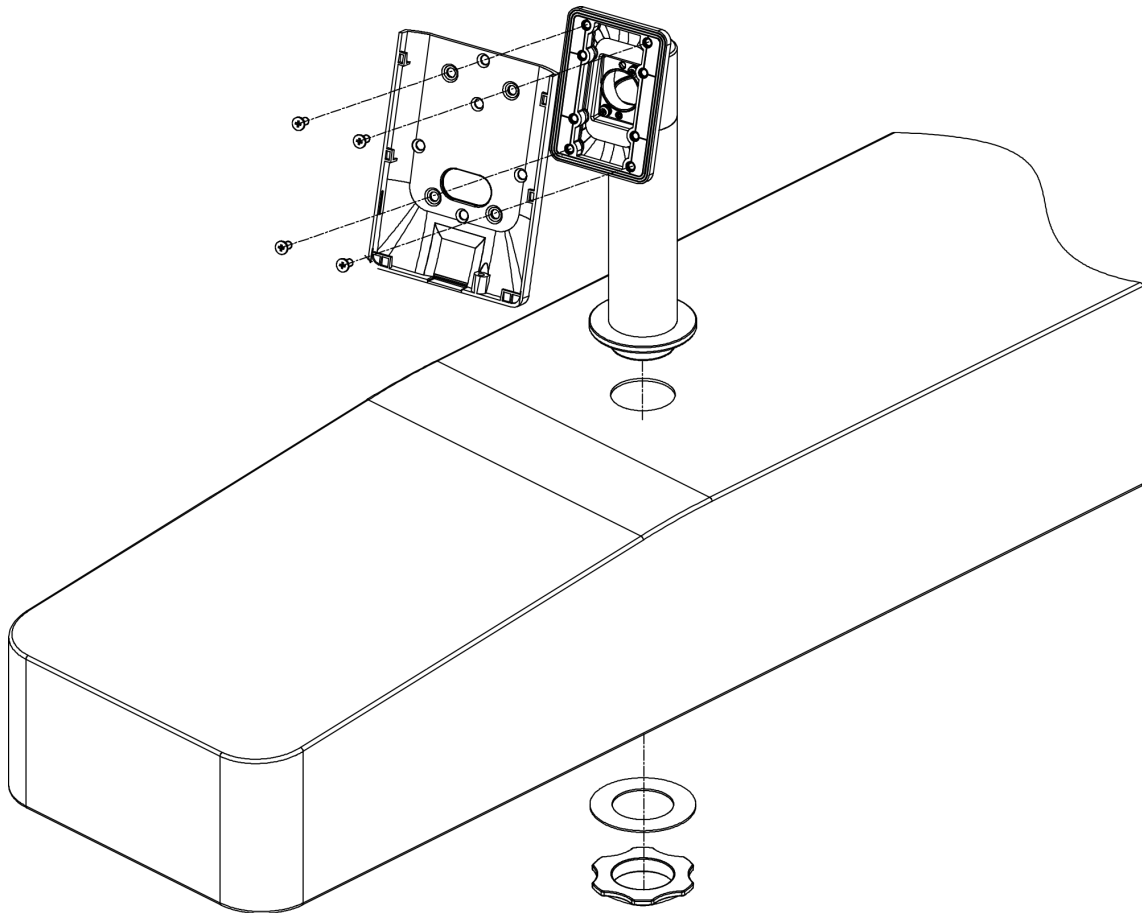
Figure 2-14 Fix Mounting Plate
