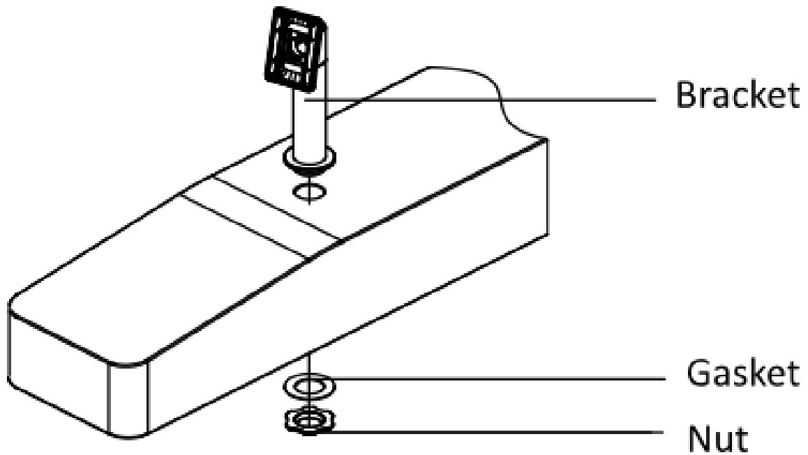
Figure 2-13 Fix Bracket
