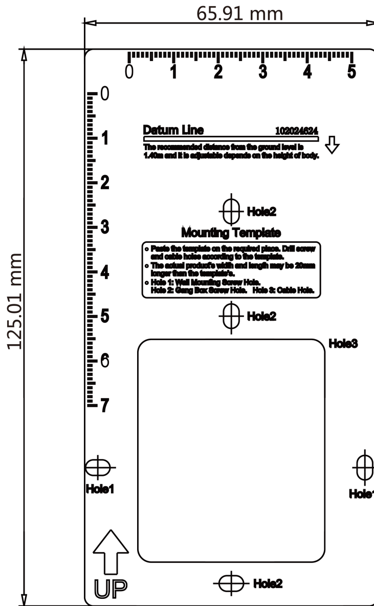
Figure 2-5 Mounting Template
