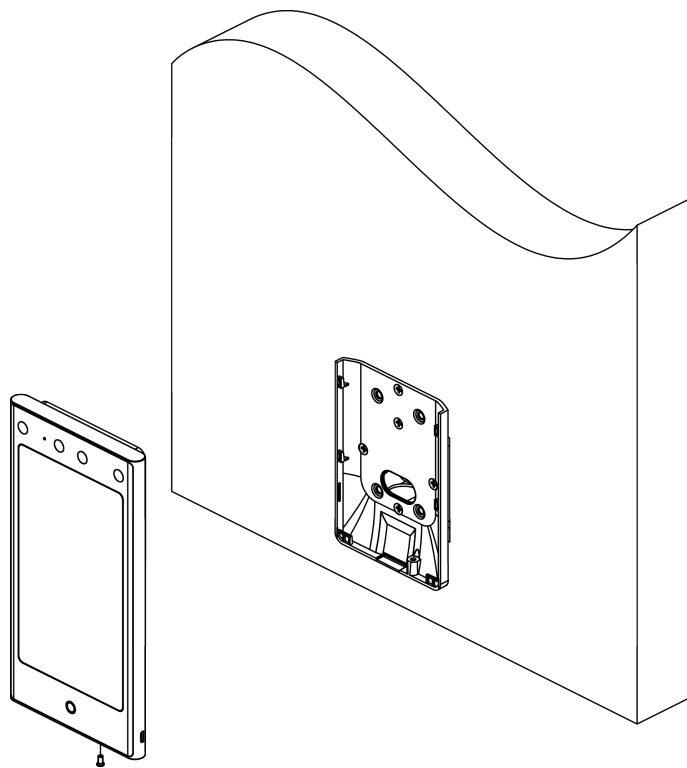
Figure 2-8 Hang Device
