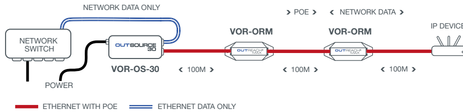
Diagram 2. Veracity's OUTSOURCE 30 provides enough power to allow 300 metres (984ft) of extension to a POE Plus wireless access point, using two OUTREACH Max devices located at 100 metre intervals.
