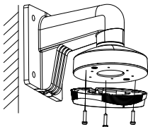
Figure 2-14 Install the Mounting Base on the Wall Mounting Bracket
