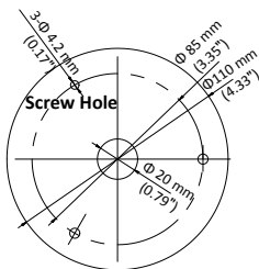
Figure 2-2 The Drill Template
