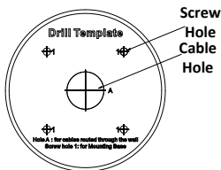
Figure 2-7 Drill Template
