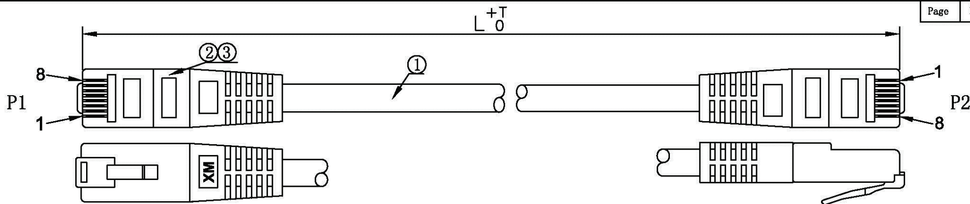
WIRING DIAGRAM
