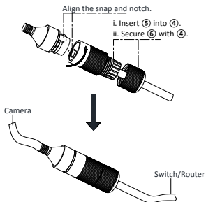
Figure 2-11 Waterproof Accessory Installation
